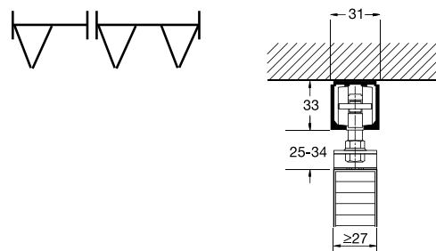
Ceiling installation Gắn trần
