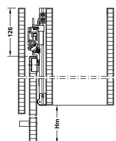
Section top view open Khi mở
