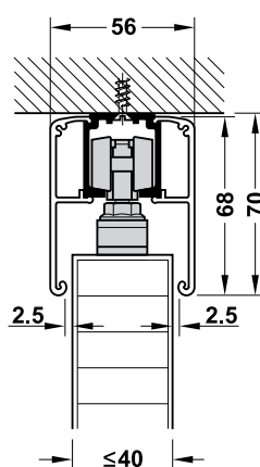
Ceiling installation Gắn trần
