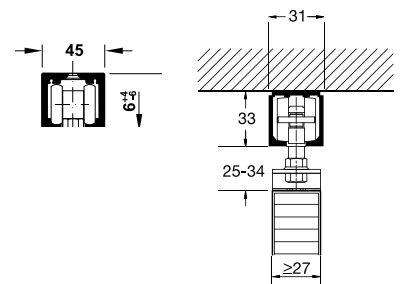
Ceiling installation Gắn trần
