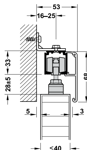
Wall installation Treo tường
