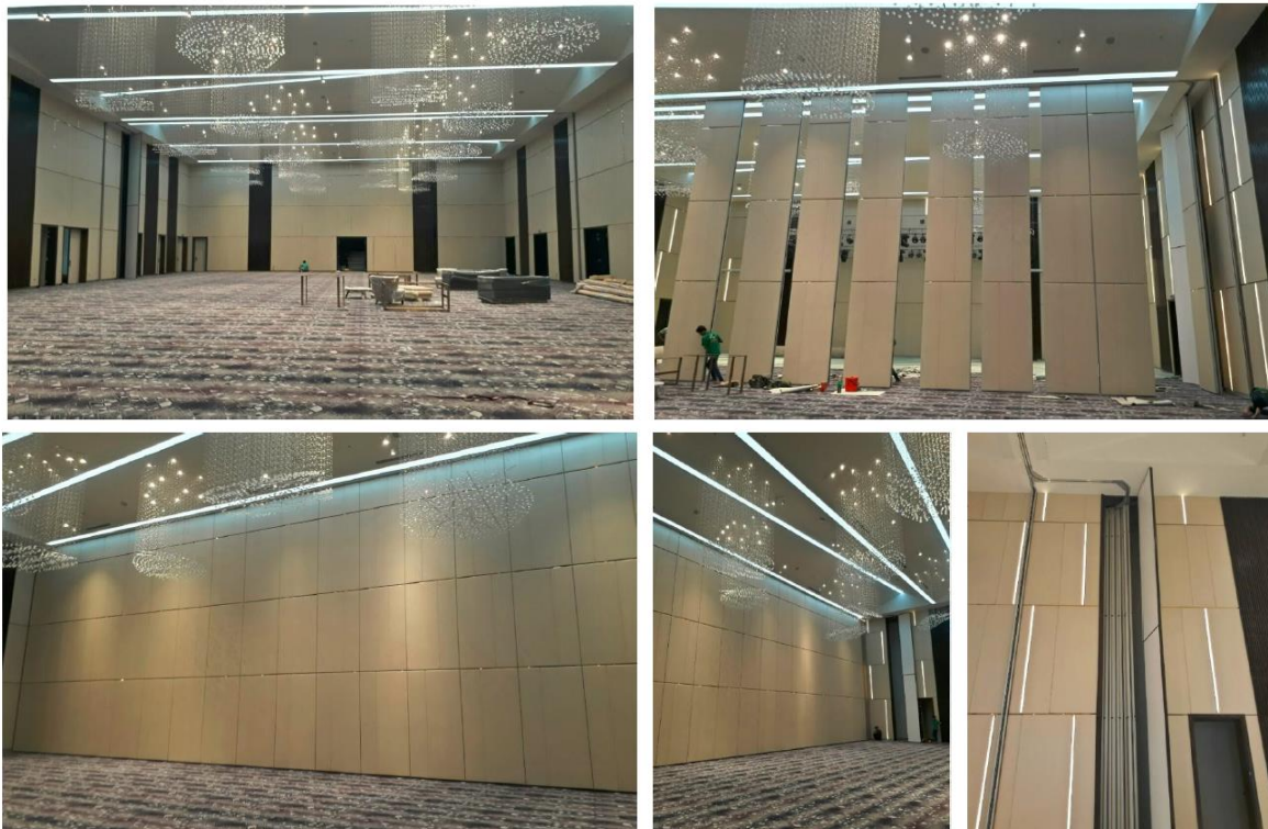
Vincom Hà Tĩnh STC 53dB, 373 SQM, H = 8.5 M
